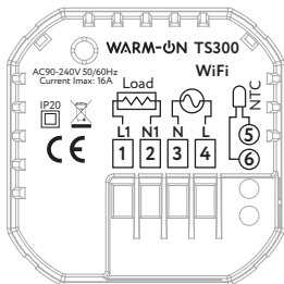
Electric Heating Wiring Diagram
